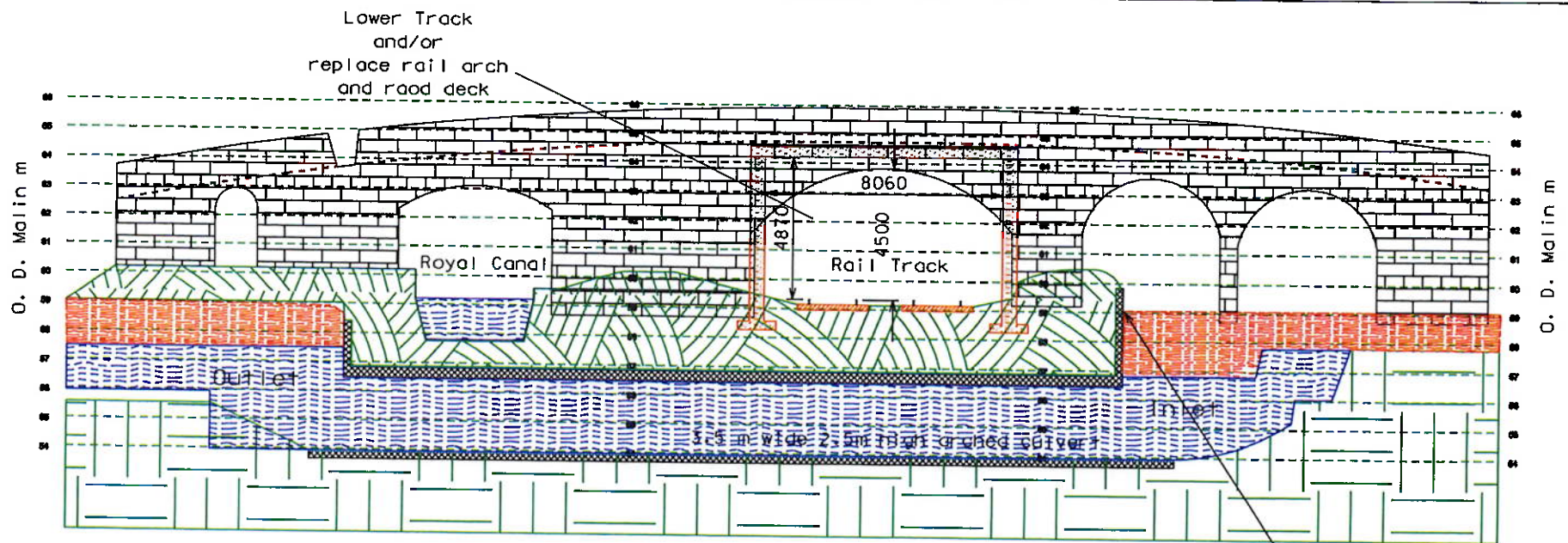
Jackson's Bridge Proposals
